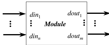
Fig. 4. Each schema may contain multiple input, din_1, \dots, din_n , and output, dout_1, \dots, dout_m , ports for unidirectional communication.
