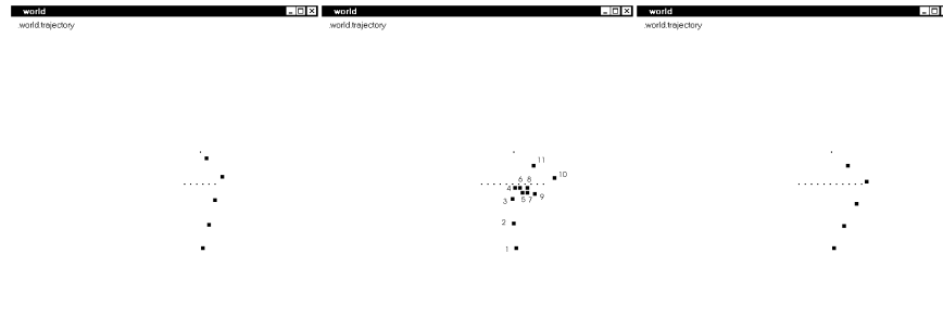
Fig. 11. The above diagrams display the Rana Comptatrix basic experiments for the prey acquisition and detour model. The different dots correspond to the frog's trajectory from its initial location as it finally reaches the prey. The left-hand side shows the resulting motion path for the 10cm barrier. Note how the frog heads directly towards the side of the barrier. The middle diagram displays the resulting motion path for the 20cm barrier experiment before learning. We have added numbers corresponding to the frog's position in time. In this particular experiment the frog hits the barrier three times before perceiving the side of the barrier and moving towards the prey. The right-hand side diagram shows the resulting motion path for the 20cm wide barrier after learning.
