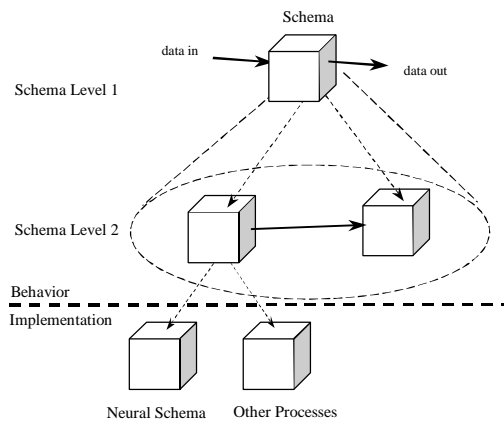
Fig. 3. The ASL/NSL computational model is based on hierarchical interconnected schemas. A schema at a higher level (level 1) is decomposed (dashed lines) into additional interconnected (solid arrow) subschemas (level 2). At the lowest level schemas are implemented by neural networks or other processes.
