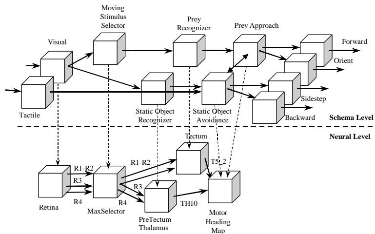
Fig. 5. Schema model hierarchy for the toad's prey acquisition and static object avoidance model previously described.
