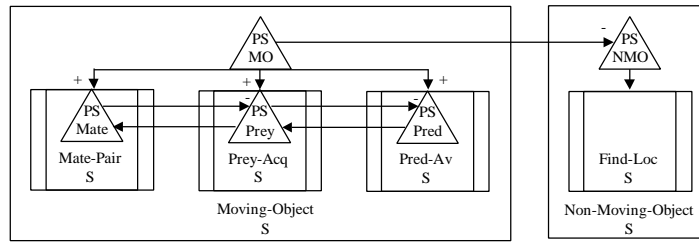
Fig. 3. Rana Computatrix ethogram: Mating, Prey Acquisition and Predator Avoidance schemas (moving and non-moving objects) [8]. The diagram shows feedback between perceptual schemas (triangles) and regular schemas (rectangles). Note the hierarchical schema organization. (Acronyms are as follows: PS - Perceptual Schema, MO - Moving Object, NMO - Non-Moving Object, S -Schemas.)
