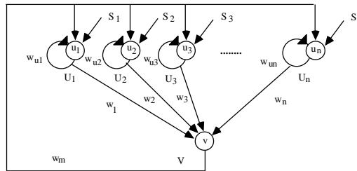
Fig. 9. The neural network shown corresponds to the architecture of the Maximum Selector model, where u_i and v represent neural membrane potentials, U_i and V represent neural firing rates, S_i represent inputs to the network, and w_i represent connection weights. The network is initialized with a number of positive inputs assigned to different cells. After many iterations the network stabilizes producing a single "winner", i.e. a single active cell.
