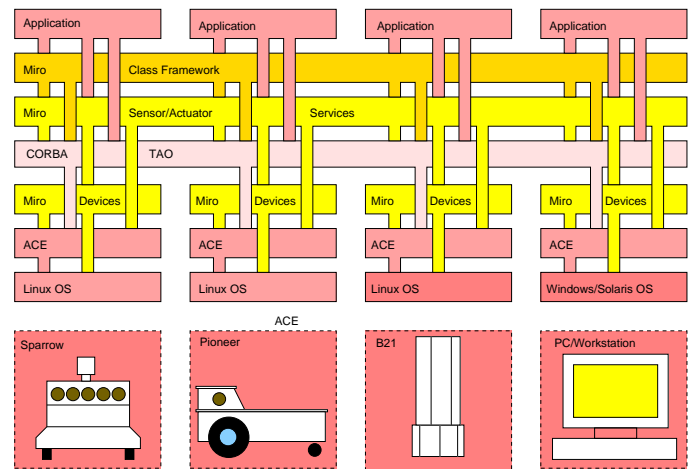
Fig. 1. The Miro architecture. The ACE and Miro device layers provide abstract interfaces for specific platforms. The TAO CORBA and Miro Service layers achieve platform-independence, network and location transparency. The Miro class framework provides classes for generic robot control functionality.
