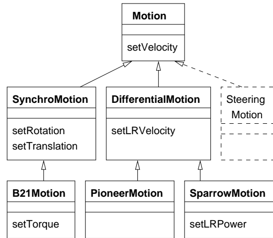
Fig. 2. Motion interface inheritance for different mobile bases.
